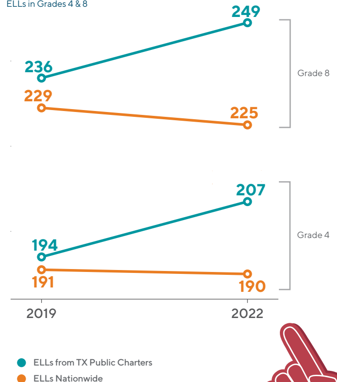
Reading Scores on NAEP Exams ELLs in Grades 4 & 8
